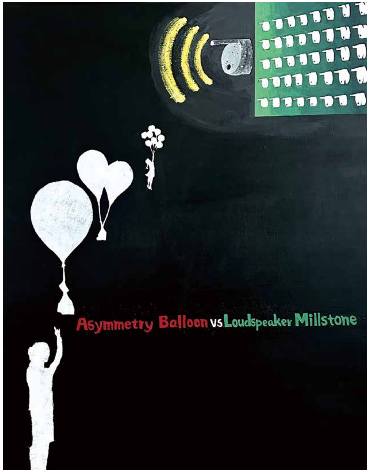
Asymmetry Balloon vs Loudspeaker Millstone
